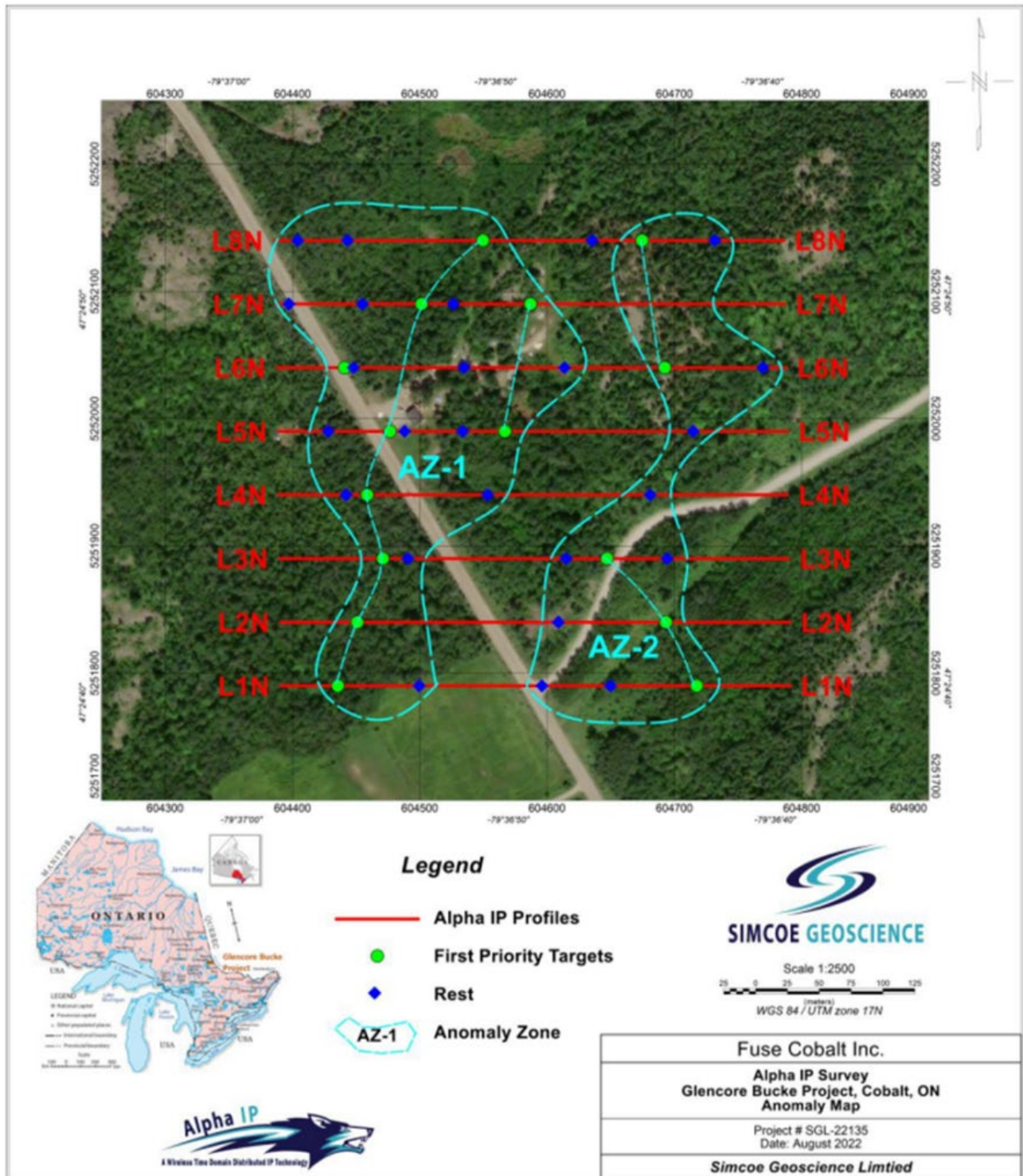
Figure 1: Overview of the Glencore Bucke area showing the Alpha IP lines, the geophysical anomalies, and potential target zones.
